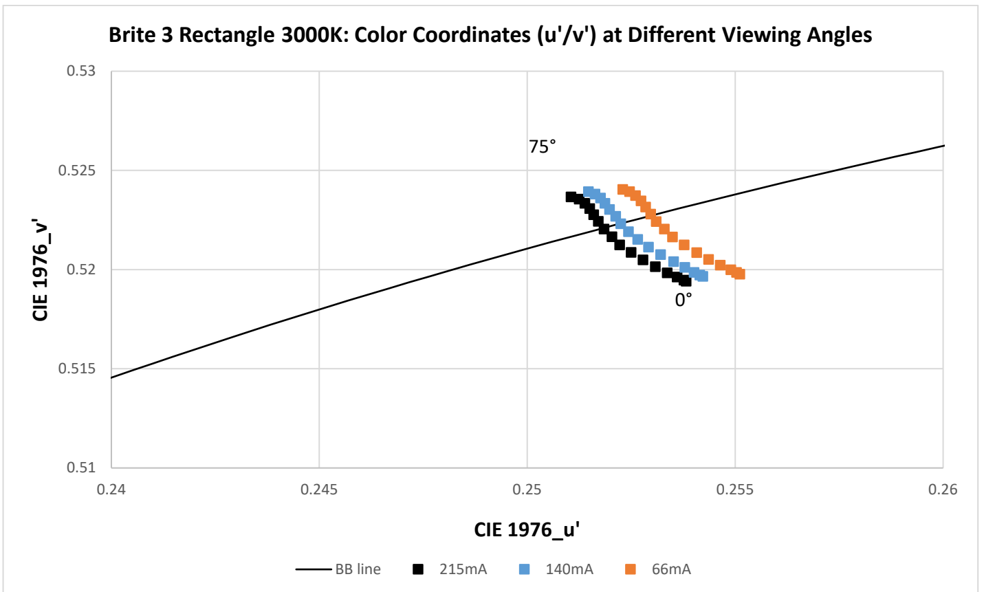
Figure 28: CIE u'/v' as function of the viewing angle. Driving currents I = 0.066\text{ A}, 0.140\text{ A}, 0.215\text{ A}, 3000\text{K}
