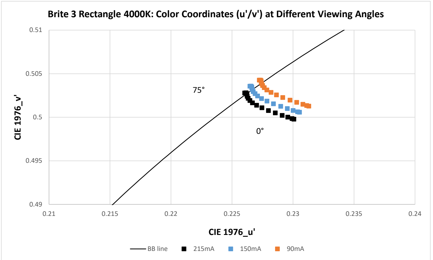
Figure 27: CIE u'/v' as function of the viewing angle. Driving currents I = 0.090\text{ A}, 0.150\text{ A}, 0.215\text{ A}, 4000\text{K}
