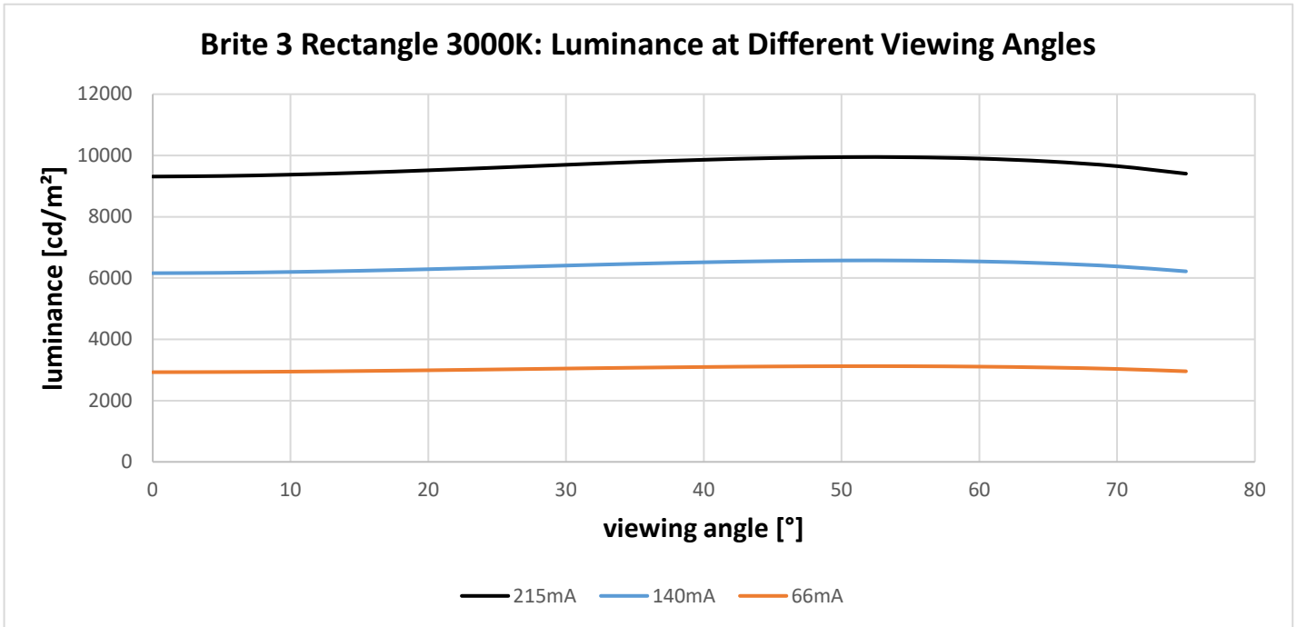
Figure 24: Luminance as function of the viewing angle. Driving currents I = 0.066 \text{ A}, 0.140 \text{ A}, 0.215 \text{ A}, 3000\text{K}
