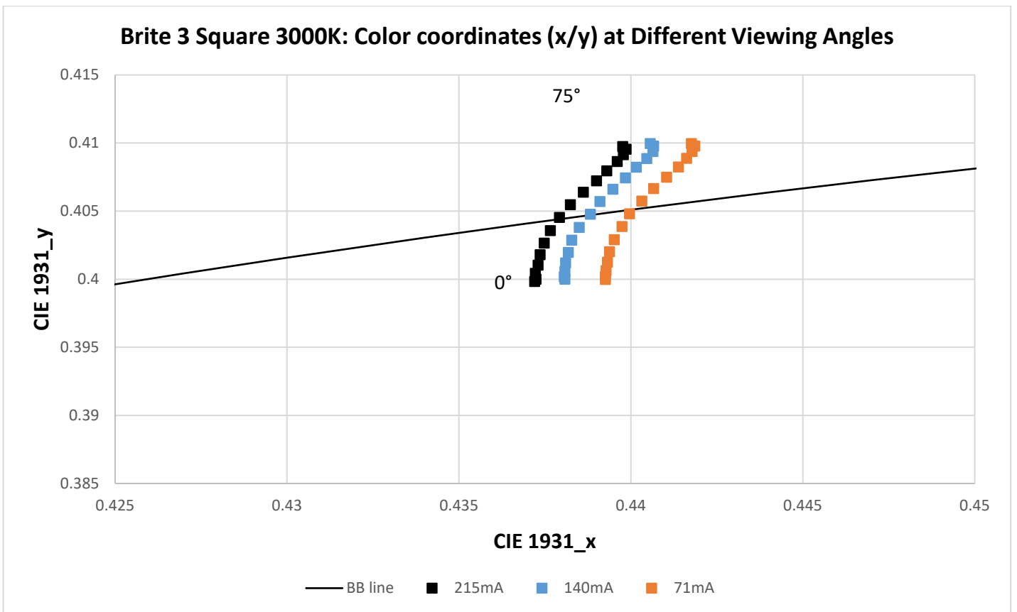
Figure 27: CIE x/y as function of the viewing angle. Driving currents I = 0.071\text{ A}, 0.140\text{ A}, 0.215 , 3000K, level 1
