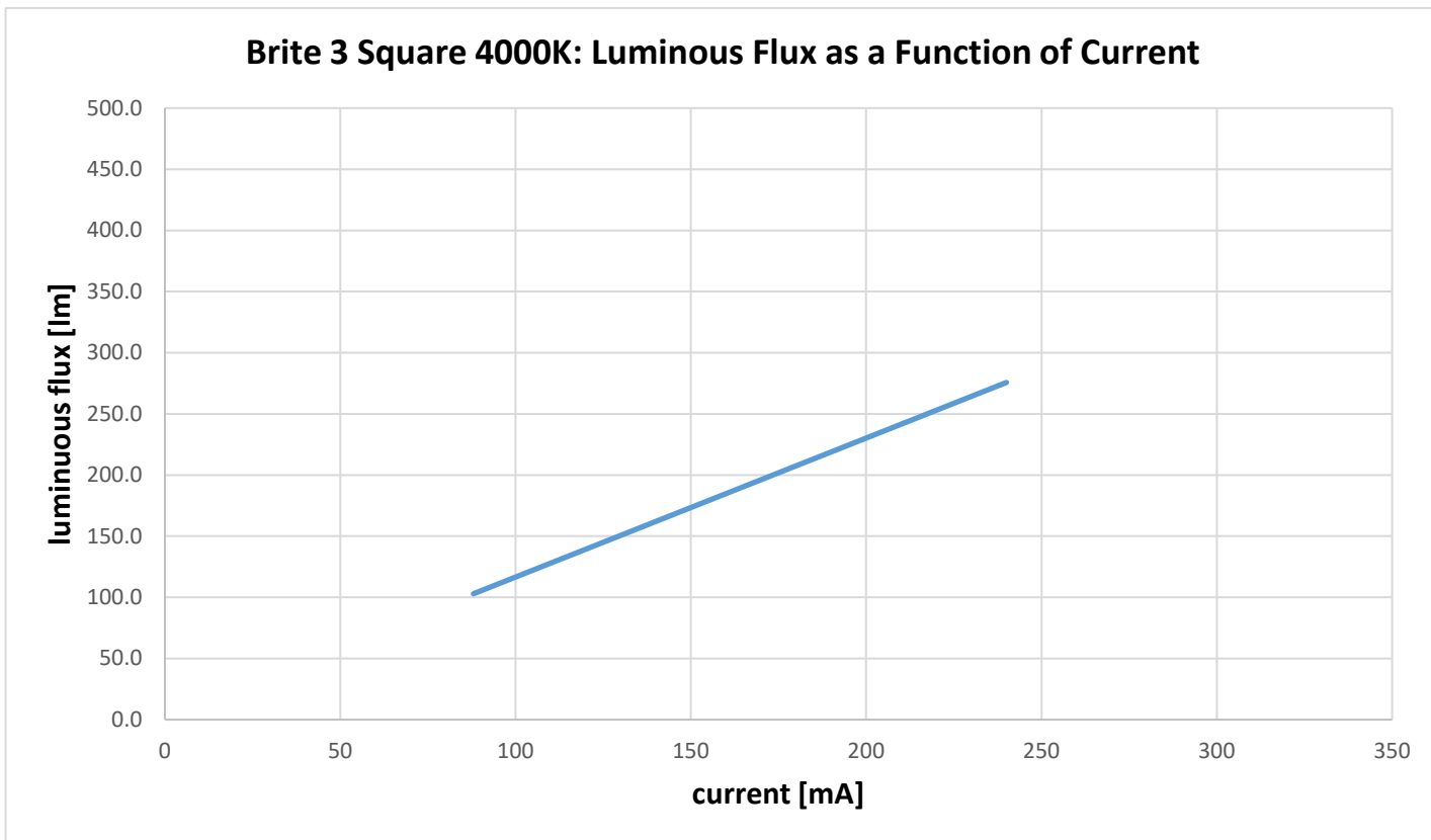
Figure 17: Luminous flux vs current, 4000K, level I
