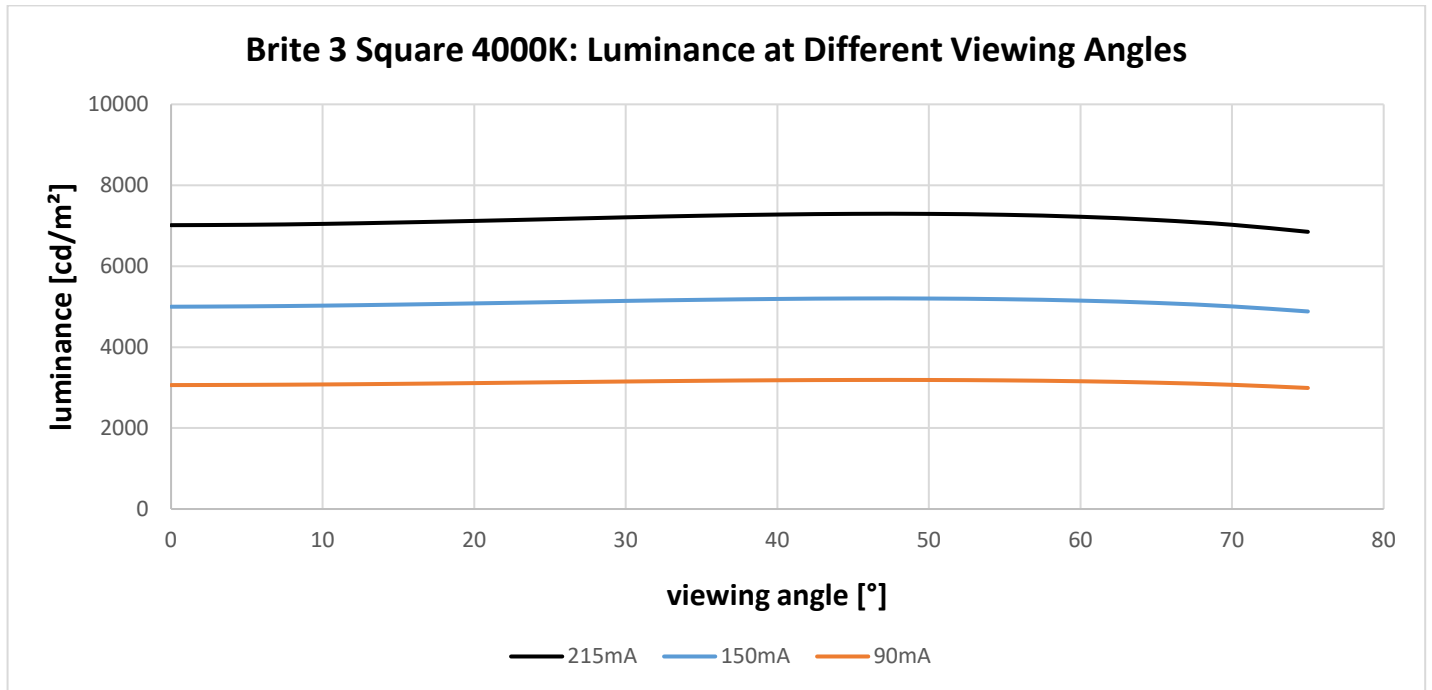
Figure 24: Luminance as function of the viewing angle. Driving currents I = 0.090 \text{ A}, 0.150 \text{ A}, 0.215 \text{ A}, 4000\text{K}
