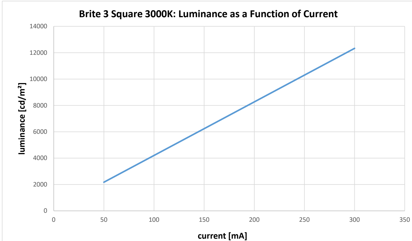
Figure 16: Luminance versus forward current at room temperature, Brite Square 3000K, level 1
