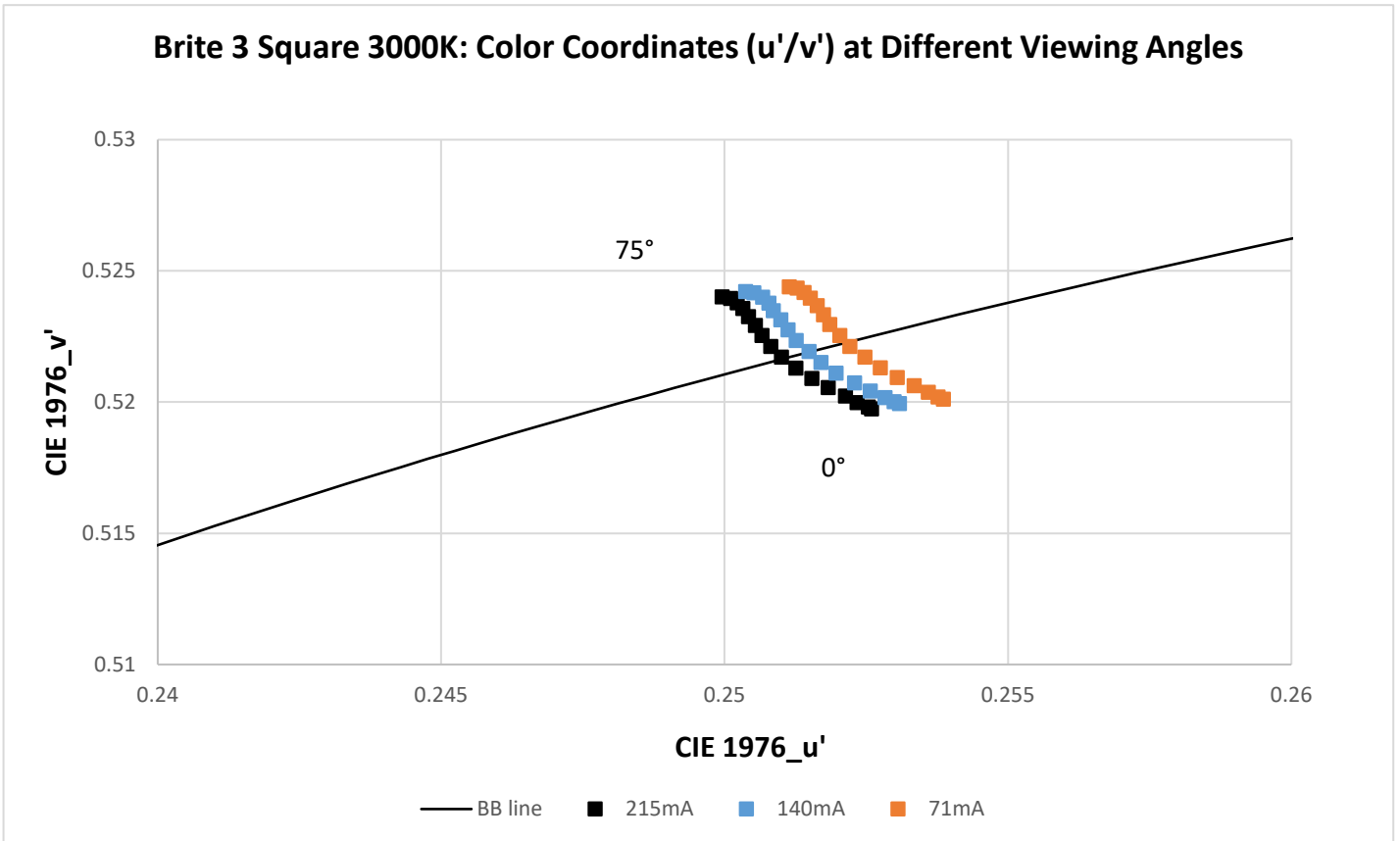
Figure 29: CIE u'/v' as function of the viewing angle. Driving currents I = 0.071\text{ A}, 0.140\text{ A}, 0.215\text{ A} , 3000K, level I
