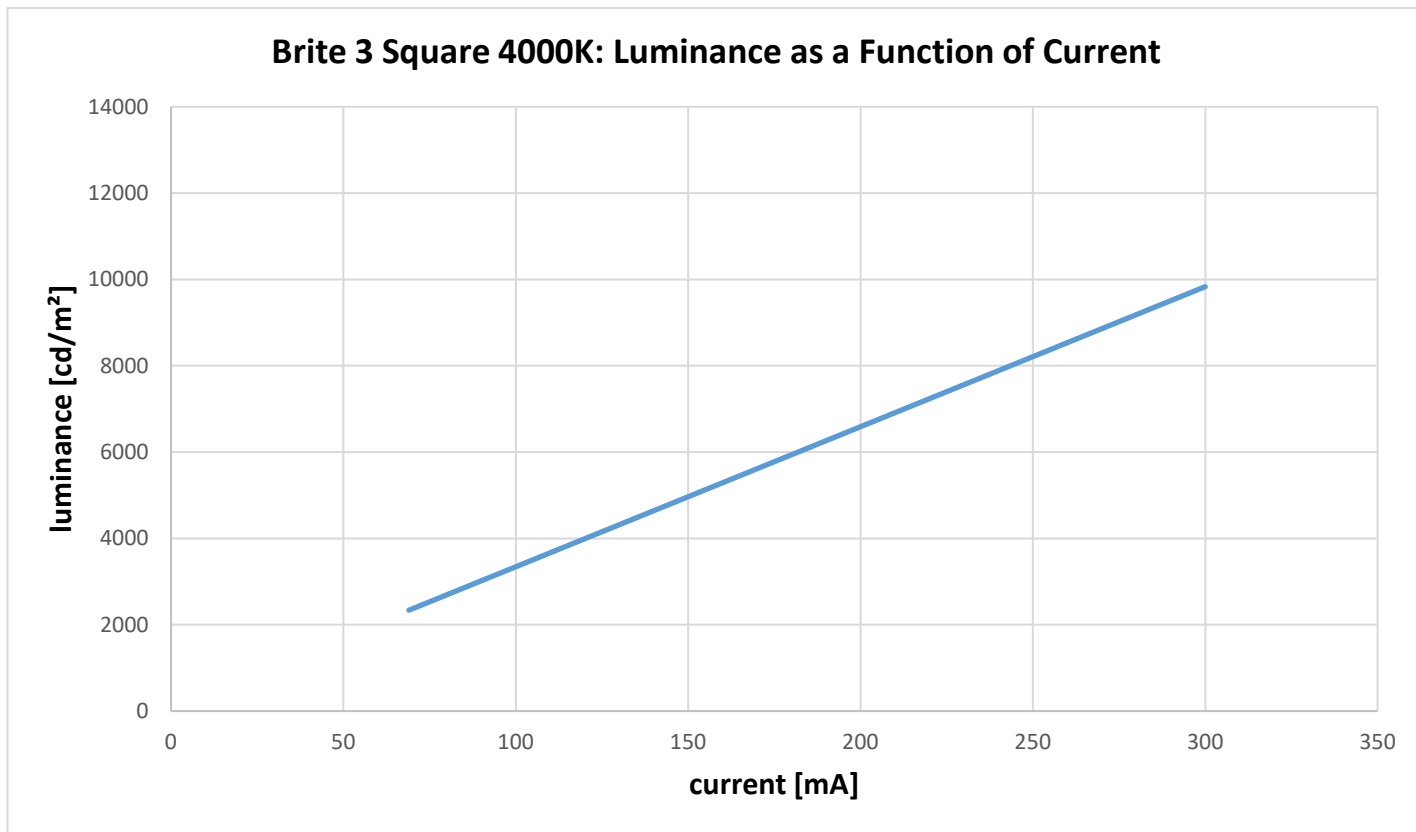
Figure 15: Luminance versus forward current at room temperature, Brite Square 4000K, level 1
