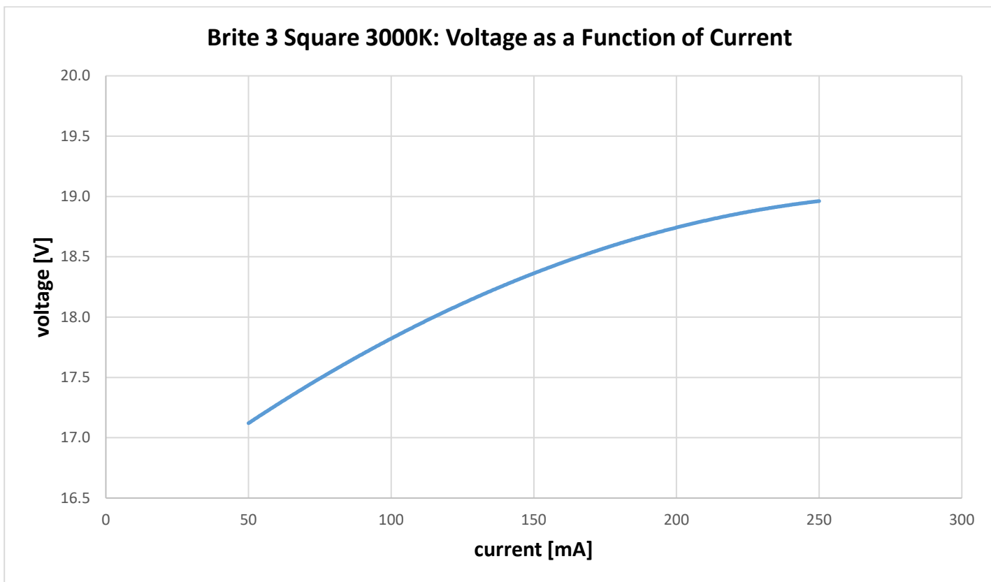
Figure 20: Voltage versus forward current at room temperature, 3000K, level 1
