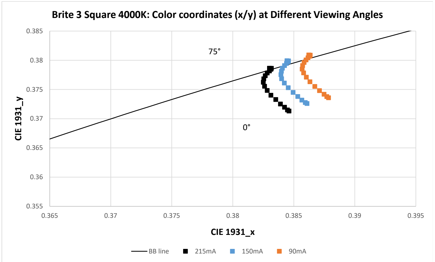
Figure 26: CIE x/y as function of the viewing angle. Driving currents I = 0.090\text{ A}, 0.150\text{ A}, 0.215\text{ A} , 4000K, level 1
