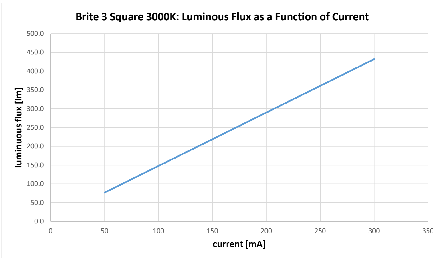
Figure 18: Luminous flux vs current, 3000K, level I
