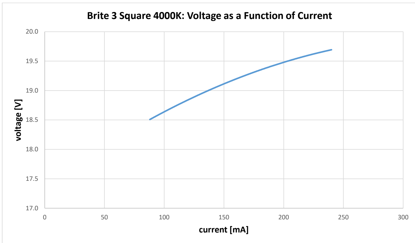
Figure 19: Voltage versus forward current at room temperature, 4000K, level 1
