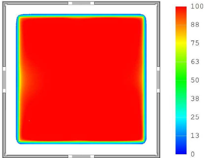
Figure 23: Typical luminance distribution for a Brite 3 Square Level 1. Operation conditions: vertical in air, RT (= 25 °C), I = I_{in rated}
