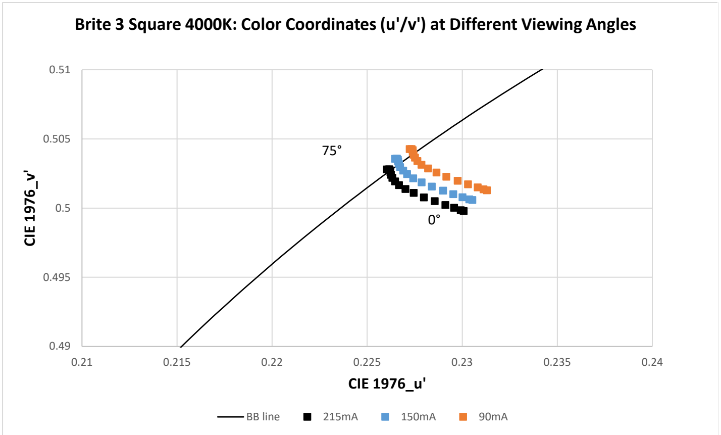
Figure 28: CIE u'/v' as function of the viewing angle. Driving currents I = 0.090\text{ A}, 0.150\text{ A}, 0.215\text{ A} , 4000K, level I
