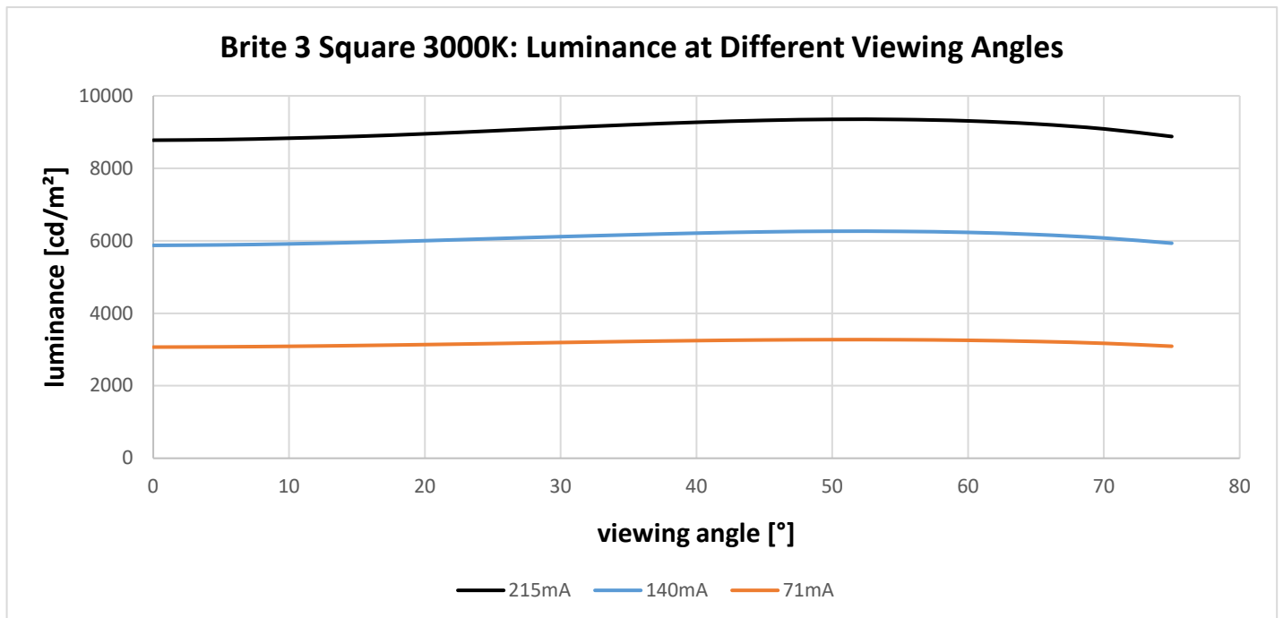
Figure 25: Luminance as function of the viewing angle. Driving currents I = 0.071 \text{ A}, 0.140 \text{ A}, 0.215 \text{ A}, 3000\text{K}
